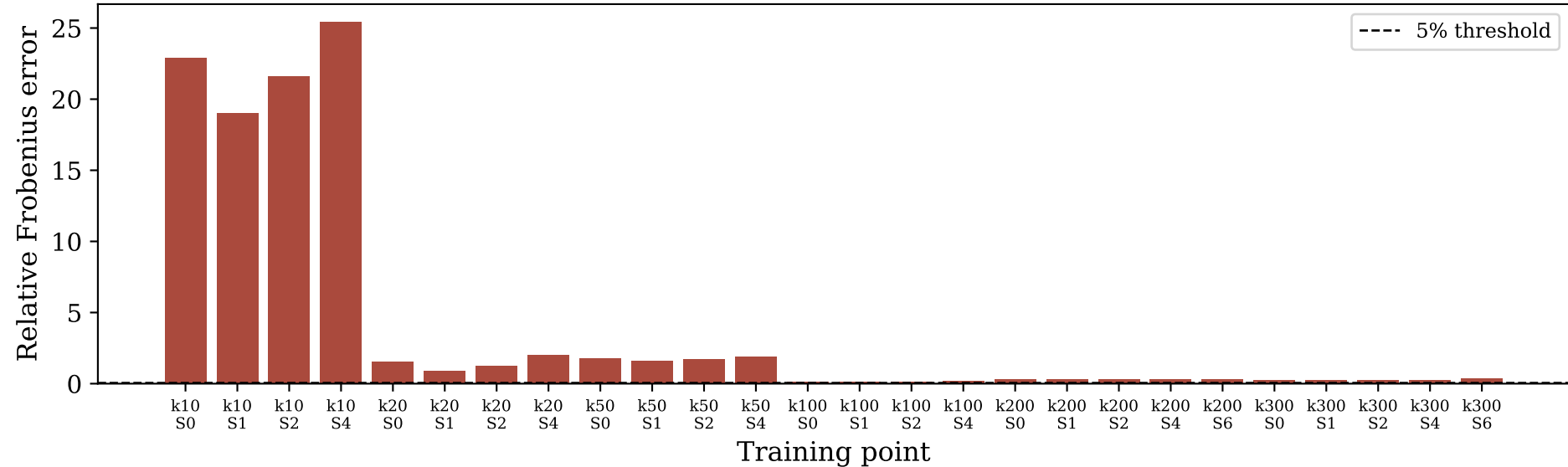
Leave-one-out interpolation error for \hat{A}
