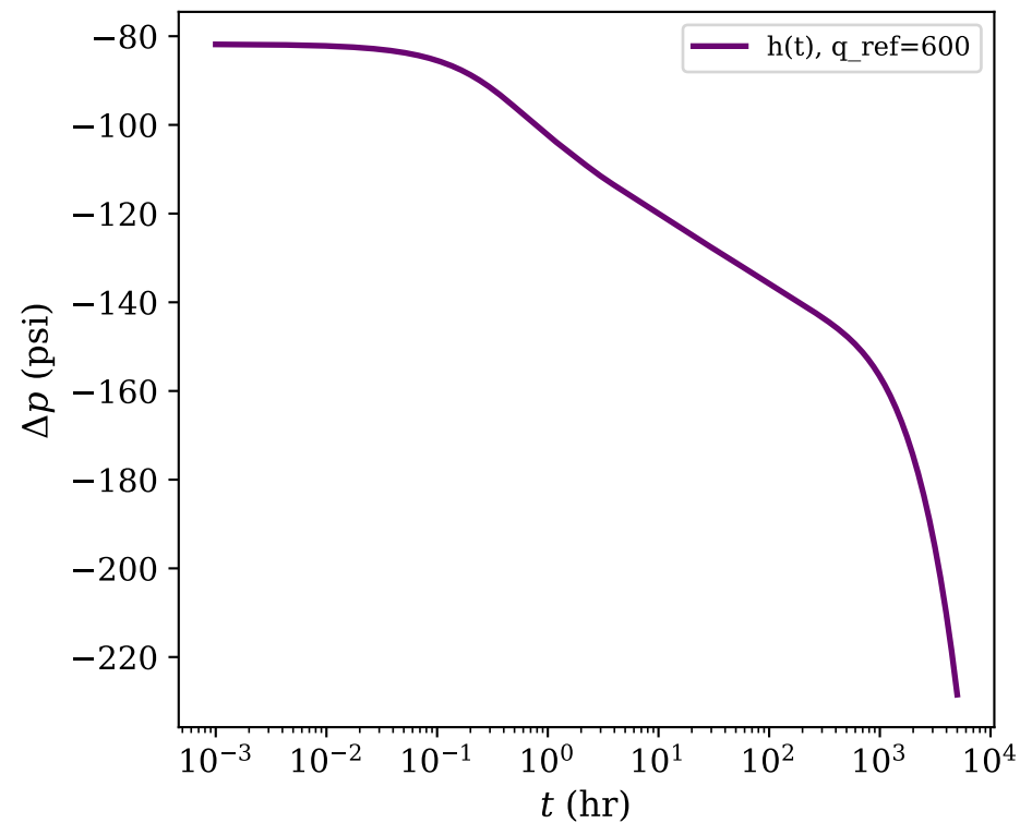
Unit Step Response k = 50 mD, S = 2
