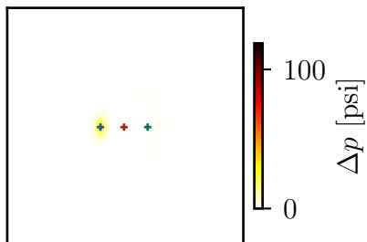
POD ( r = 6 ) \varepsilon_G = 0.0131\%
