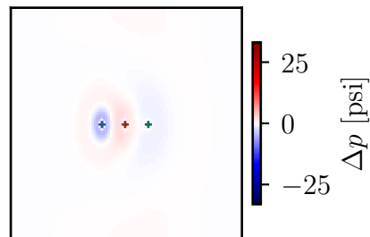
Residual ( r = 6 ) Max \Delta : 33.07 psi
