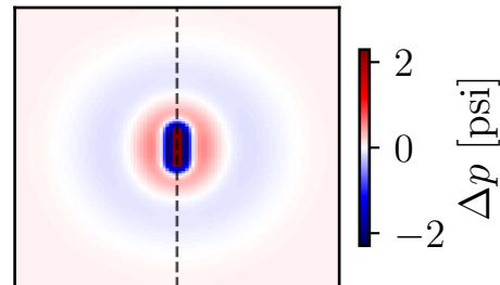
Residual ( r = 4 ) Max \Delta : 2.29 psi
