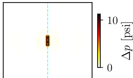
POD ( r = 6 ) \varepsilon_G = 0.0021\%
