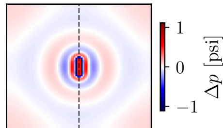
Residual ( r = 6 ) Max \Delta : 1.11 psi
