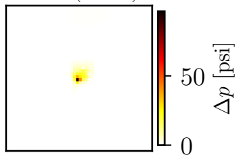
POD ( r = 4 )
