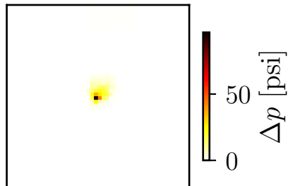
POD ( r = 4 ) \varepsilon_G = 0.0070\%
