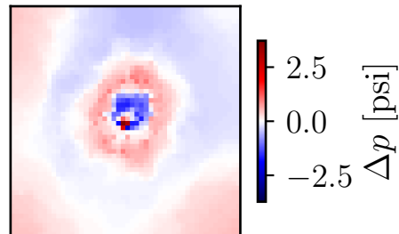
Residual ( r = 4 ) Max \Delta : 3.72 psi
