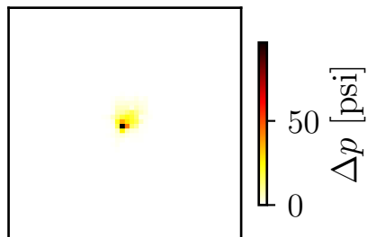
POD ( r = 6 ) \varepsilon_G = 0.0032\%
