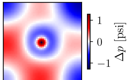
Residual ( r = 3 ) Max \Delta : 1.28 psi
