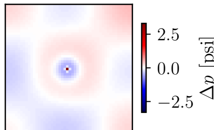
Residual ( r = 3 ) Max \Delta : 3.30 psi
