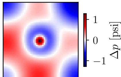
Residual ( r = 3 ) Max \Delta : 1.28 psi
