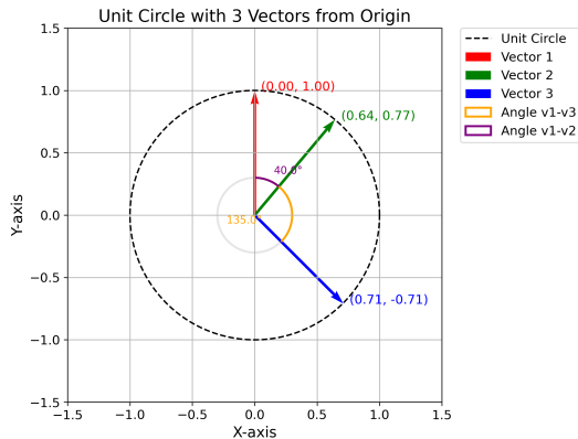
Cosine similarity of vectors
