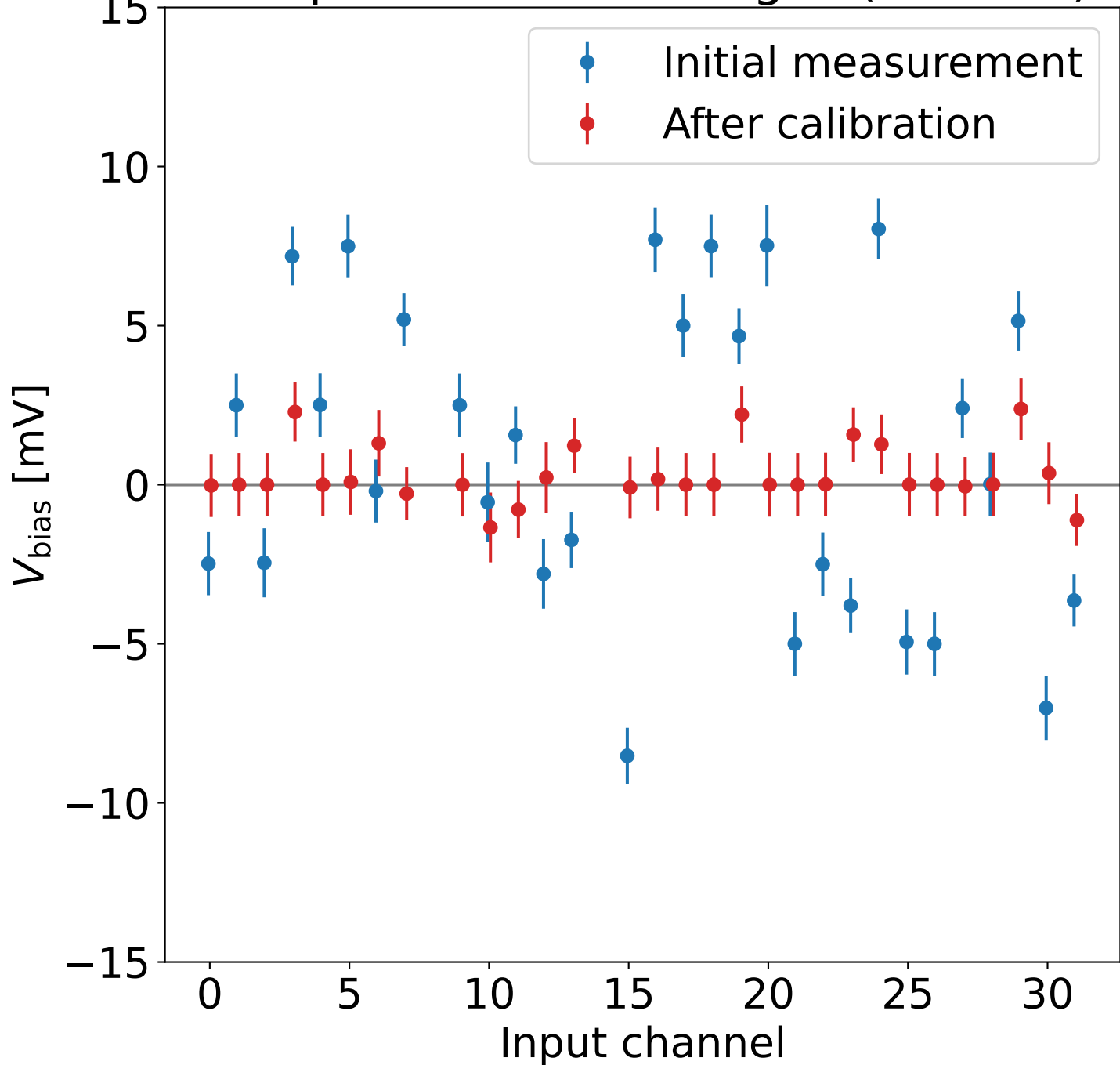
Comparator bias voltages (Board 1)
