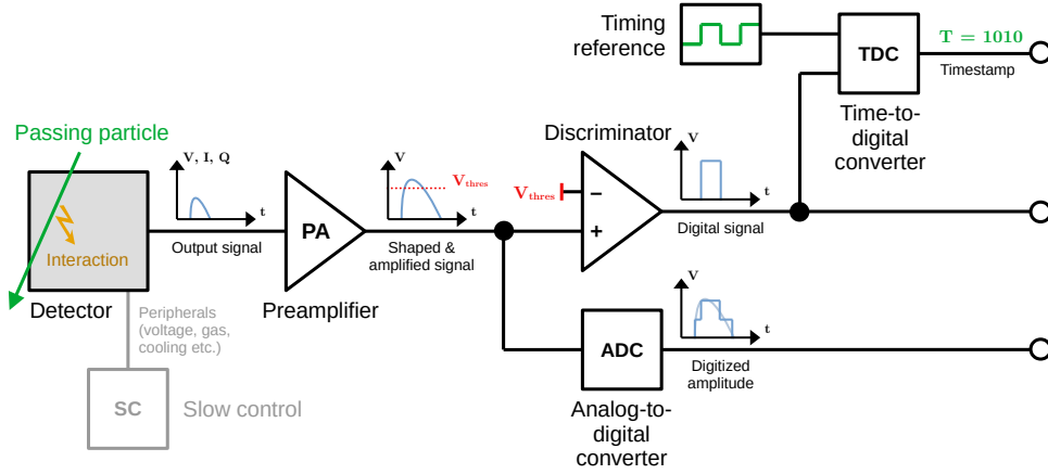
Fig. 3.7: Schematic overview of an electronic readout chain of a particle detector. The detector output signal is shaped and amplified in the preamplifier. After that, several components can be connected. The discriminator outputs a digital signal if the detector signal is above a certain threshold. The digital signal can then be converted to a timestamp with a TDC. Alternatively, the analog signal can be digitized with an ADC [29, adapted].
