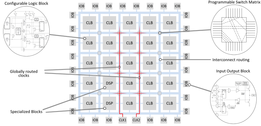
Fig. 3.8: Illustration of the internal structure of an FPGA. The fabric consists of a matrix of CLBs with programmable interconnections. IOBs on the chip edges allow interfacing to the external pins [46].
