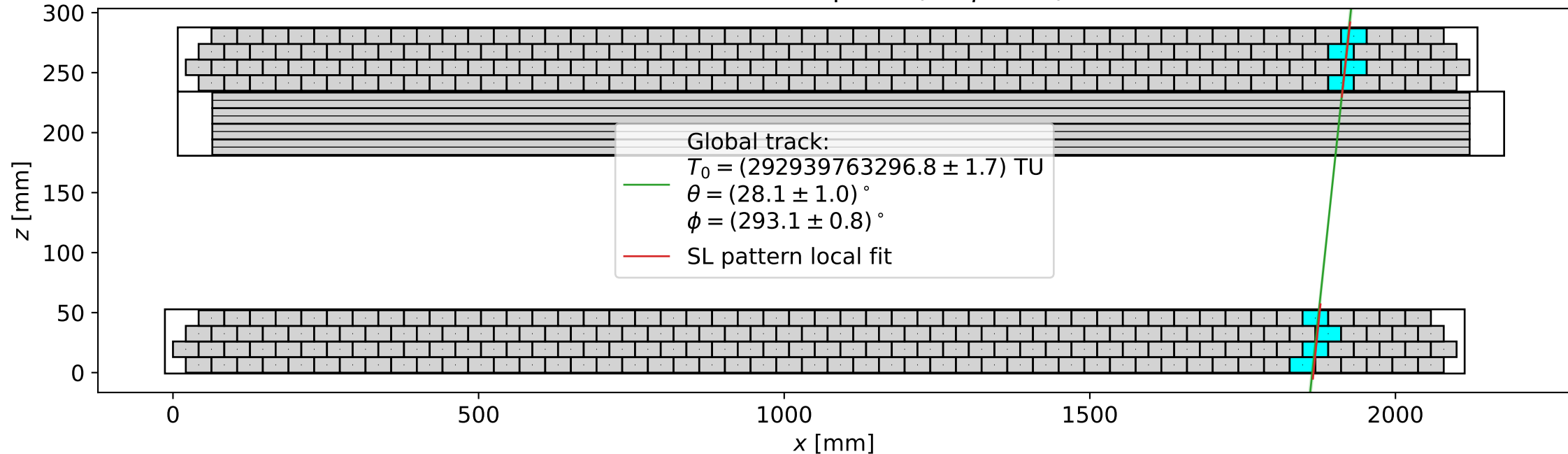
Global track: x-z-plane (SL- \phi view)
