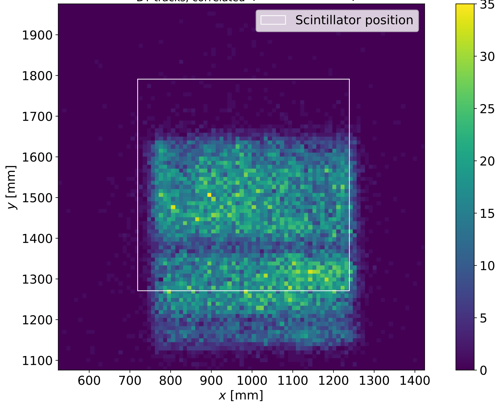
N_{\text{DT}} tracks, correlated ( z = -965\text{mm} )
