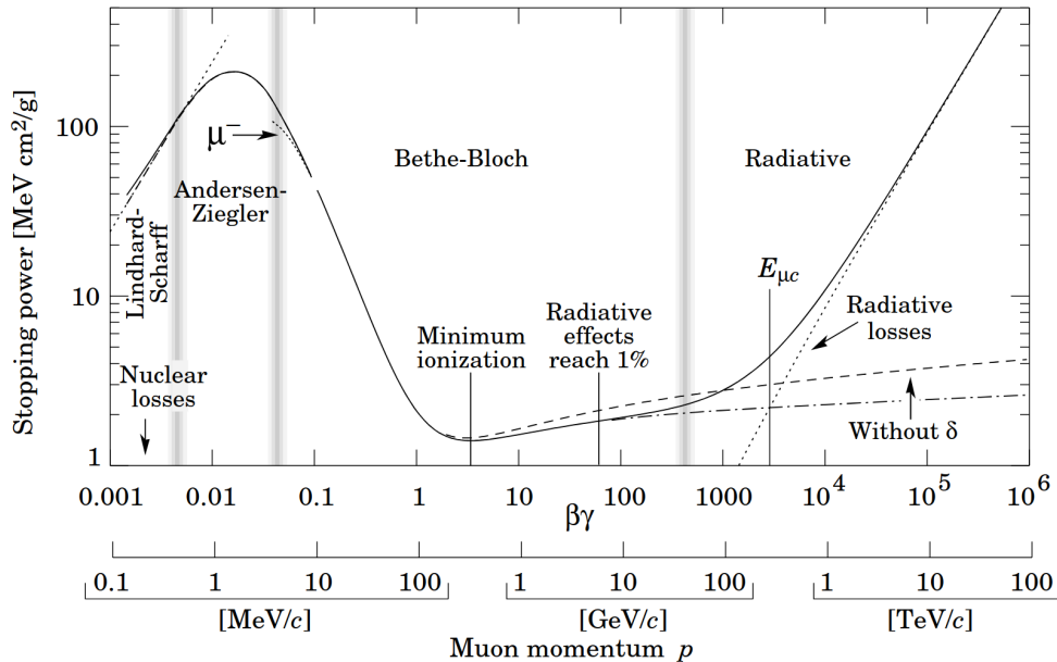
Fig. 3.1: Stopping power for antimuons ( \mu^+ ) in copper depending on the momentum [8].
