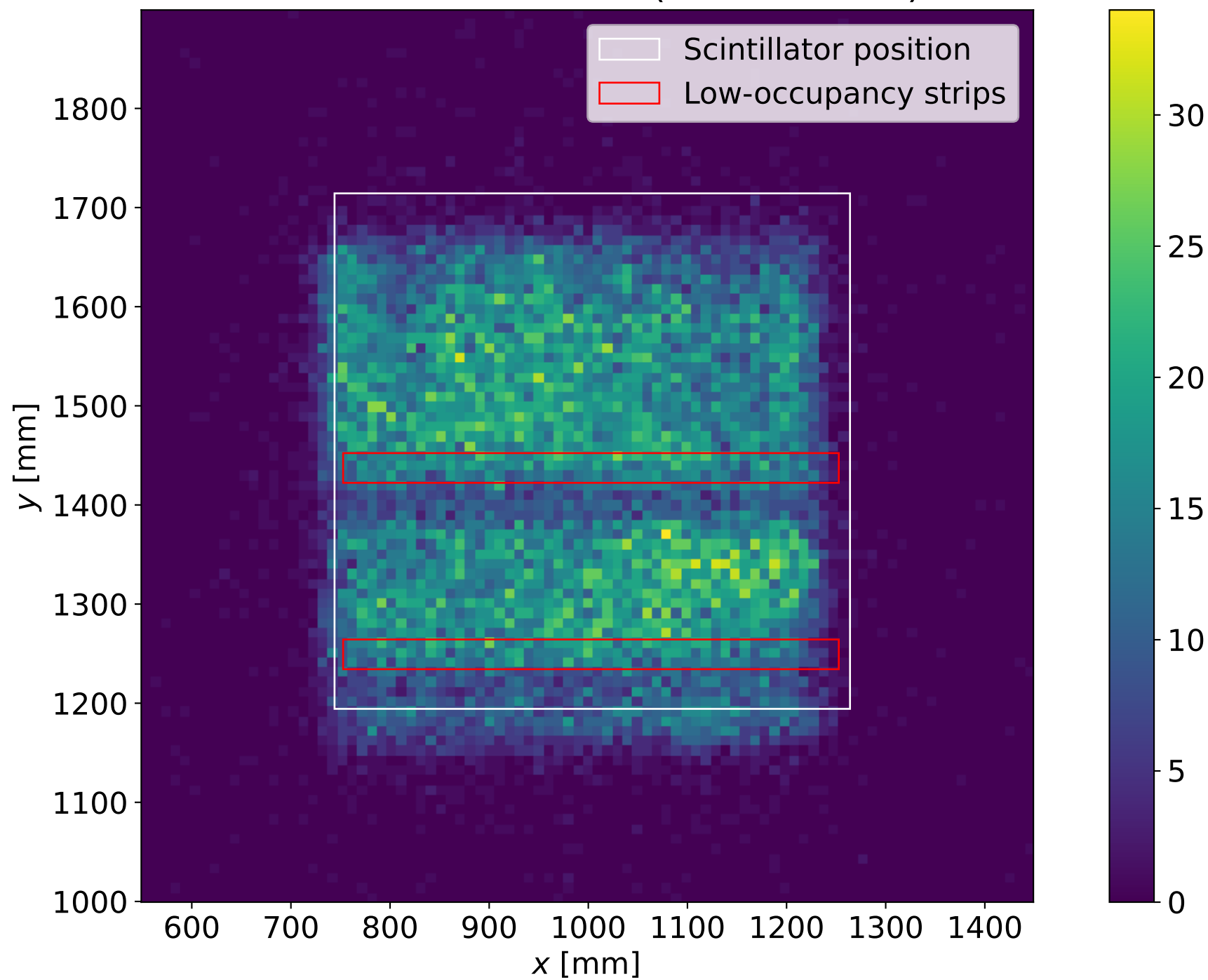
Correlated DT tracks ( z = -966\text{mm} )
