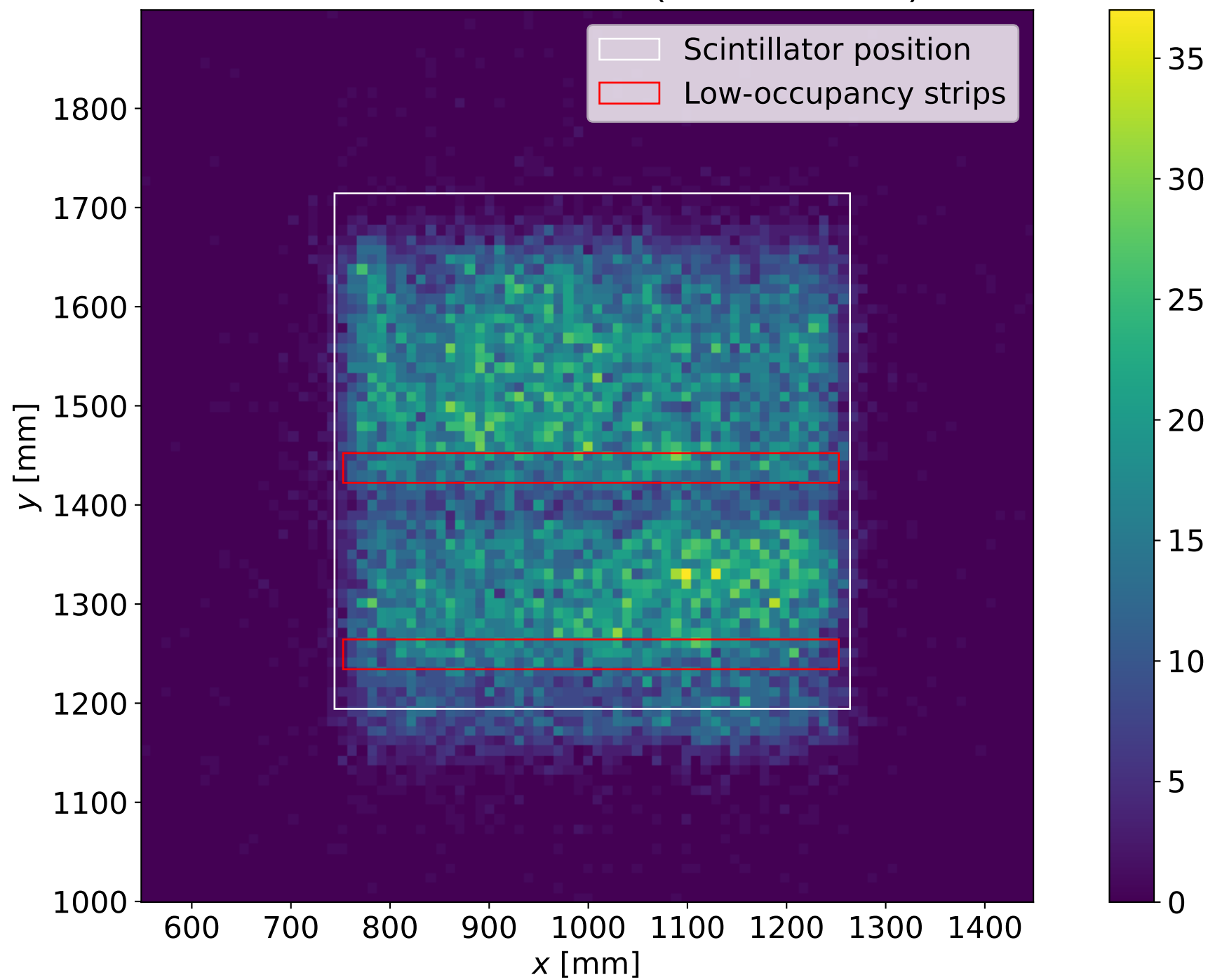
Correlated DT tracks ( z = -926\text{mm} )
