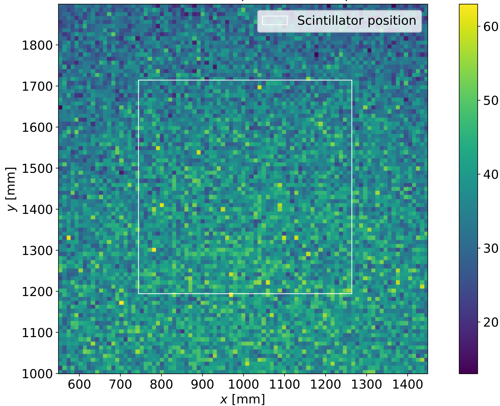
All DT tracks ( z = -926\text{mm} )
