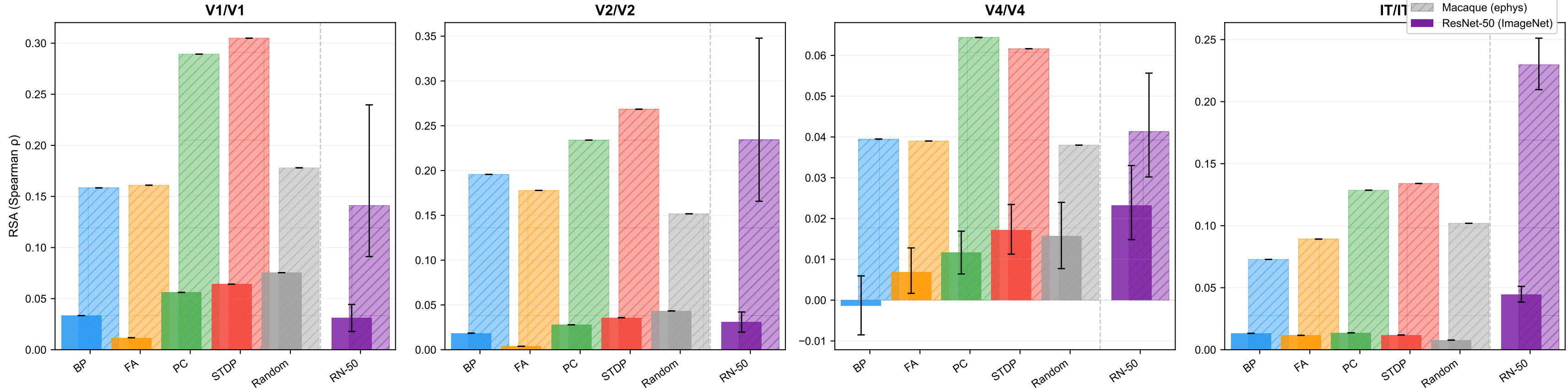
Architecture Comparison: Custom 3-conv CNN (learning rules) vs ResNet-50 Pretrained
