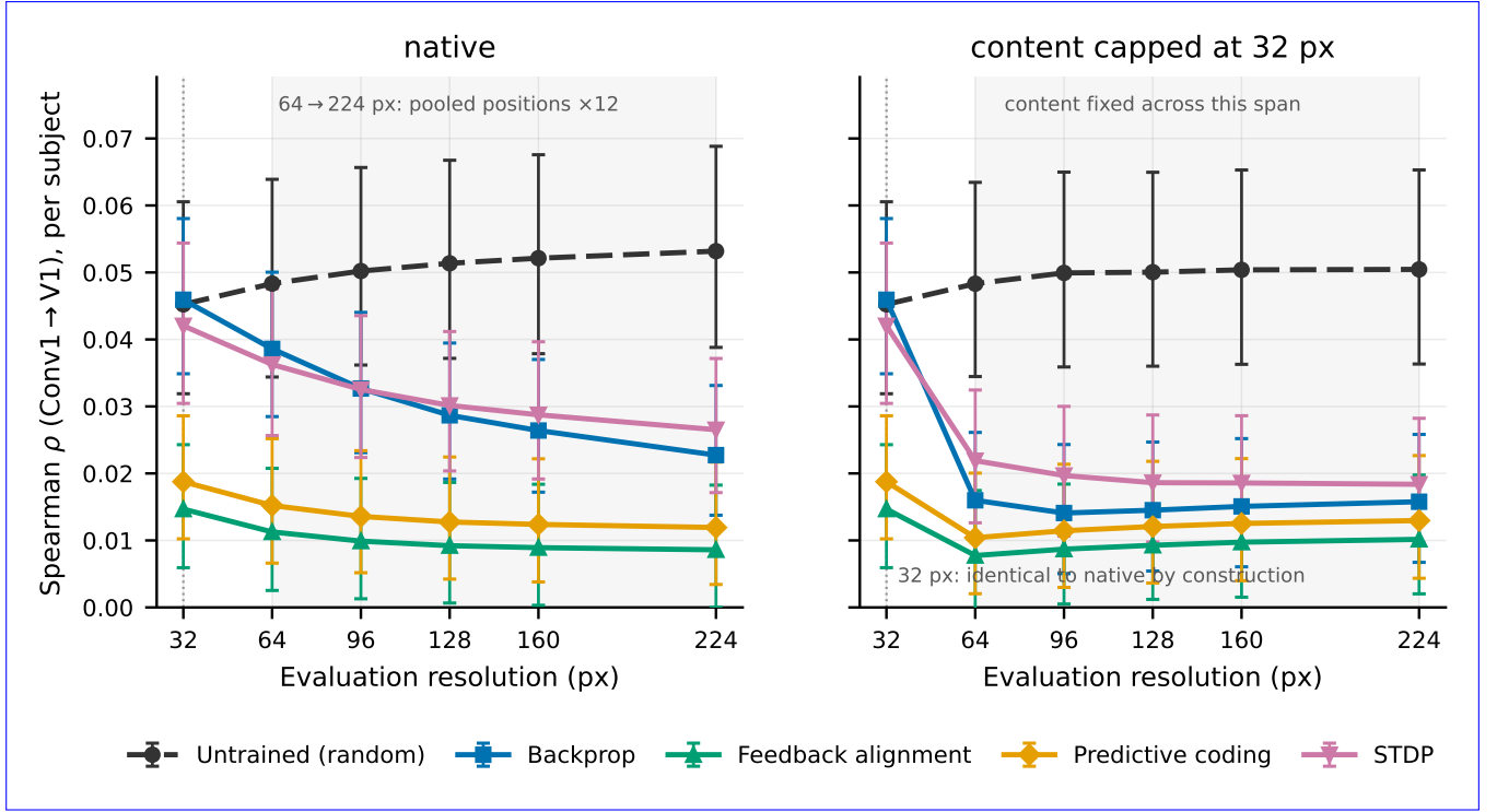
Figure 5: The dependence is on image content, not on pooled positions. With image content limited to the training resolution, the V1 gap is as large as with native content. V1 alignment (Conv1 \rightarrow V1) vs. evaluation resolution, mean \pm SEM over 5 seeds with 95% stimulus-bootstrap CIs (per subject, cross-run pairs), with stimuli at their native resolution (left) and with their content capped at 32px before upsampling (right). The arms are identical at 32 px by construction. What differs is the shape. At native resolution the trained conditions decline steadily across the whole sweep; with content fixed-limited they drop once at the first step, where-as soon as the resize-chain-is-introduced input exceeds the training resolution, and then run flat or turn-back-up . Across the shaded 64 \rightarrow 224px span the pooled positions increase twelvefold while the right-hand arm's content stays fixed, and the Random-Backprop gap opens by +0.003 +0.002 there against +0.030 +0.021 on the left. Only the untrained network rises in both arms.
