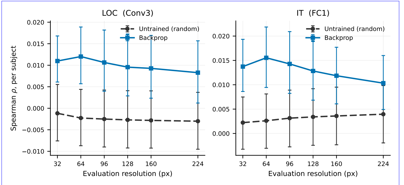
Figure 7: A genuine learning effect survives at higher areas. Backprop vs. untrained alignment ( \pm SEM per subject, cross-run pairs: 95% stimulus-bootstrap CIs , 5 seeds) across resolution at LOC (left) and IT (right). Backprop exceeds the untrained baseline at every resolution (5/5 seeds), unlike at V1.
