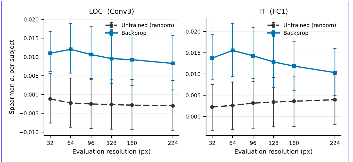
Figure 7: A genuine learning effect survives at higher areas. Backprop vs. untrained alignment ( \pm SEM per subject, cross-run pairs: 95% stimulus-bootstrap CIs , 5 seeds) across resolution at LOC (left) and IT (right). Backprop exceeds the untrained baseline at every resolution (5/5 seeds), unlike at V1.
