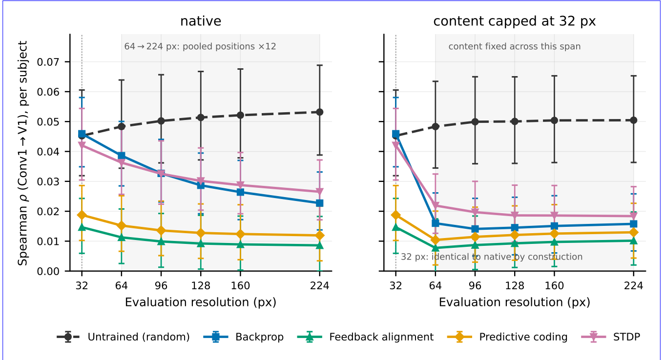
Figure 5: With image content limited to the training resolution, the V1 gap is as large as with native content. V1 alignment (Conv1 \rightarrow V1) vs. evaluation resolution, mean over 5 seeds with 95% stimulus-bootstrap CIs (per subject, cross-run pairs), with stimuli at their native resolution (left) and with their content capped at 32 px before upsampling (right). The arms are identical at 32 px by construction. What differs is the shape. At native resolution the trained conditions decline steadily across the whole sweep; with content limited they drop at the first step, as soon as the input exceeds the training resolution, and then run flat. Across the shaded 64 \rightarrow 224 px span the pooled positions increase twelvefold while the right-hand arm's content stays fixed, and the Random–Backprop gap opens by +0.002 there against +0.021 on the left. Only the untrained network rises in both arms.
