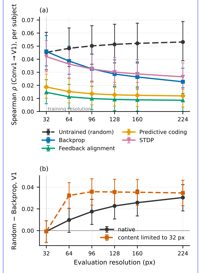
Figure 1: V1 alignment is a function of evaluation resolution. (a) Mean Spearman \rho (Conv1 \rightarrow V1, per subject, cross-run pairs) across 5 seeds, with 95% stimulus-bootstrap CIs. Every trained condition peaks at the 32px training resolution and declines; only the untrained random network rises. The Random-Backprop gap is \approx 0 at 32px and grows to +0.030 at 224px; the same pattern holds, shifted downward, after low-level statistics are partialled out (§3.4). (b) Random-Backprop gap, paired per seed and averaged over the 5 seeds, with paired 95% stimulus-bootstrap CIs, for native stimuli and for stimuli with content limited to 32px (§3.5).
