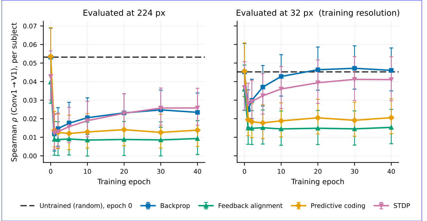
Figure 6: “Training degrades V1” tracks the same dependence. V1 alignment (Conv1 \rightarrow V1) over training, evaluated at 224px (left) and at the 32 px training resolution (right), mean across-over seeds and subjects of per-subject \rho on cross-run pairs, with 95% stimulus-bootstrap CIs . At 224 px backprop appears to degradedrops in the first epoch and recovers only partly ; at 32 px it returns to baseline, showing no net degradation.
