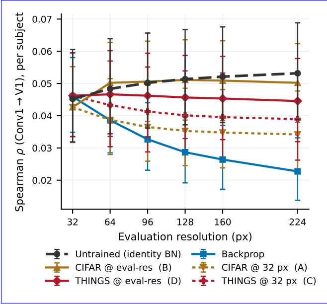
Figure 2: The effect is not the untrained baseline’s normalization. V1 alignment vs. evaluation resolution for the untrained network with its initialized (identity) batch-normalization statistics and for four calibrated variants ( 2 \times 2 : CIFAR-10 or disjoint THINGS images, at 32 px or at the evaluation resolution), with the backprop-trained network for reference. Calibration leaves the convolutional weights bit-identical. Resolution-matched calibration costs little and preserves the untrained network’s V1 advantage over backprop.
