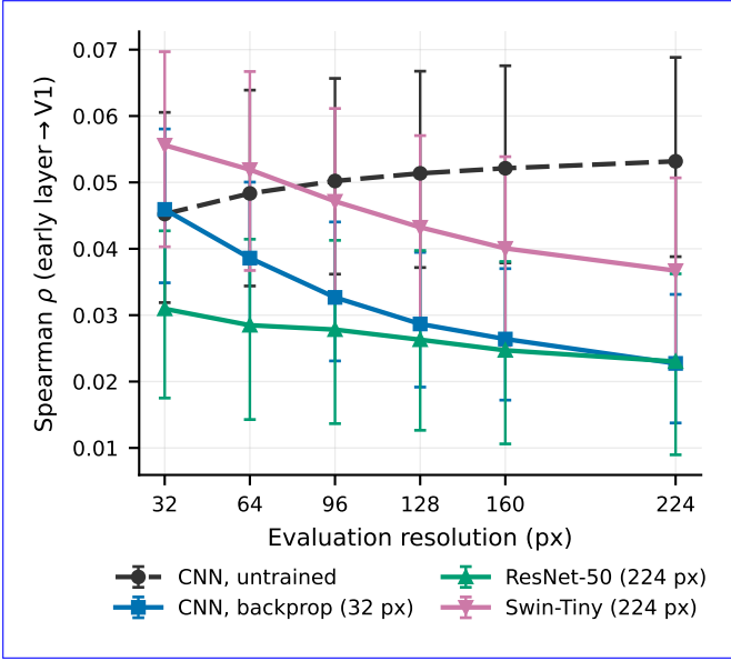
Figure 3: Architecture-independent, not train/eval matching. V1 alignment vs. evaluation resolution for three architecture families. All three trained models, including ResNet-50 and Swin-Tiny (both trained at 224 px), fall toward 224 px; only the untrained CNN rises. There is no crossover at the 224 px training resolution.
