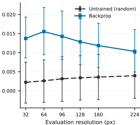
IT (FC1)
