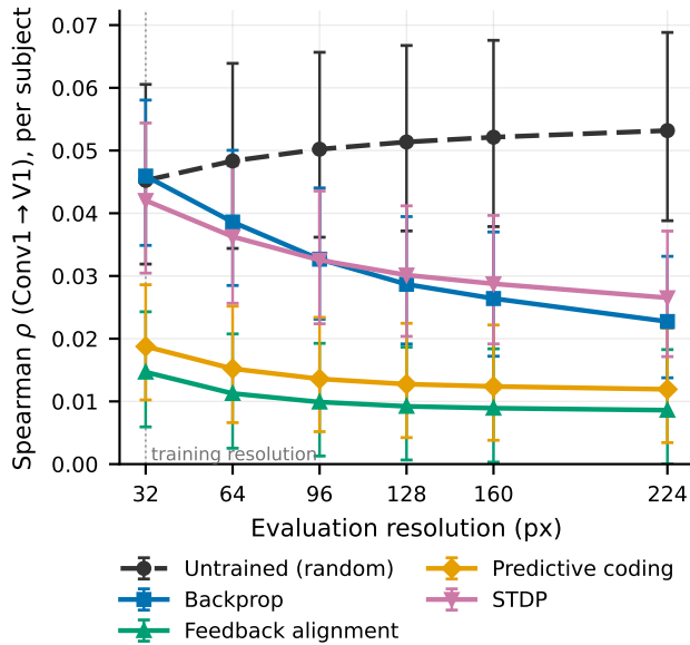
Figure 1: V1 alignment is a function of evaluation resolution. Mean Spearman \rho (Conv1 \rightarrow V1, per subject, cross-run pairs) across 5 seeds, with 95% stimulus-bootstrap CIs. Every trained condition peaks at the 32px training resolution and declines; only the untrained random network rises. The Random–Backprop gap is \approx 0 at 32px and grows to +0.030 at 224px; the same pattern holds, shifted downward, after low-level statistics are partialled out (§3.4).
