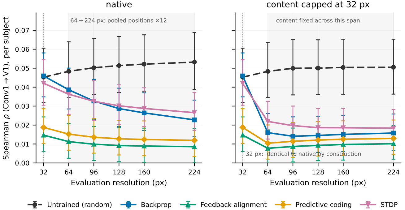
Figure 5: The dependence is on image content, not on pooled positions. V1 alignment (Conv1 \rightarrow V1) vs. evaluation resolution, mean over 5 seeds with 95% stimulus-bootstrap CIs (per subject, cross-run pairs), with stimuli at their native resolution (left) and with their content capped at 32px before upsampling (right). The arms are identical at 32px by construction. What differs is the shape. At native resolution the trained conditions decline steadily across the whole sweep; with content fixed they drop once at the first step, where the resize chain is introduced, and then run flat or turn back up. Across the shaded 64 \rightarrow 224px span the pooled positions increase twelvefold while the right-hand arm’s content stays fixed, and the Random–Backprop gap opens by +0.002 there against +0.021 on the left. Only the untrained network rises in both arms.
