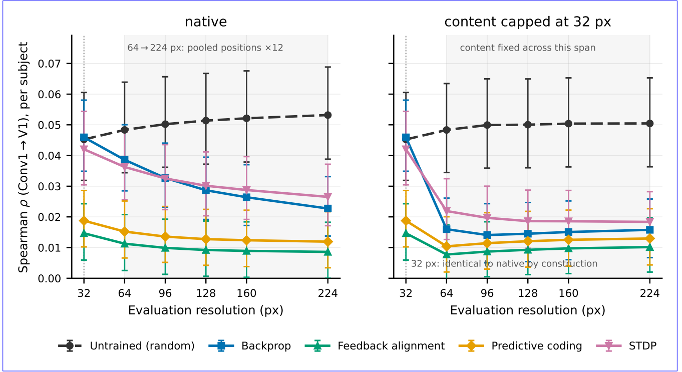
Figure 5: The dependence is on image content, not on pooled positions. With image content limited to the training resolution, the V1 gap is as large as with native content. V1 alignment (Conv1→V1) vs. evaluation resolution, mean \pm SEM over 5 seeds with 95% stimulus-bootstrap CIs (per subject, cross-run pairs), with stimuli at their native resolution (left) and with their content capped at 32px before upsampling (right). The arms are identical at 32px by construction. What differs is the shape. At native resolution the trained conditions decline steadily across the whole sweep; with content fixed-limited they drop once at the first step, where-as soon as the resize-chain-is-introduced input exceeds the training resolution, and then run flat or turn-back-up . Across the shaded 64 → 224px span the pooled positions increase twelvefold while the right-hand arm’s content stays fixed, and the Random–Backprop gap opens by +0.003 +0.002 there against +0.030 +0.021 on the left. Only the untrained network rises in both arms.
