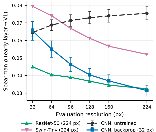
Figure 3: Architecture-independent, not train/e-val matching. V1 alignment vs. evaluation resolution for three architecture families. All three trained models, including ResNet-50 and Swin-Tiny (both trained at 224 px), fall toward 224 px; only the untrained CNN rises. There is no crossover at the 224 px training resolution.
