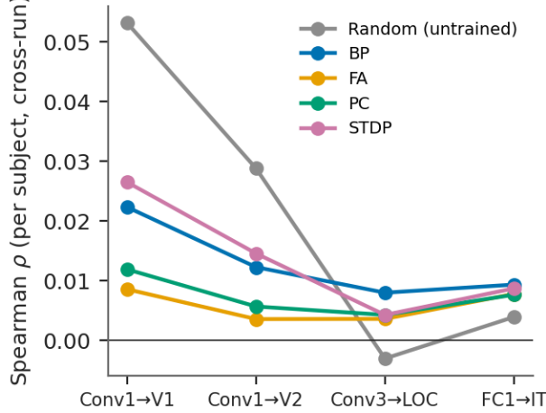
Figure 4: Brain alignment along the fixed layer-to-ROI mapping ( \rho_{\text{subj}} , cross-run). All conditions are lower at LOC than at V1. At IT the conditions lie between 0.004 and 0.009 and are not distinguishable. The untrained network is the highest at V1/V2 and the lowest at LOC and IT.
