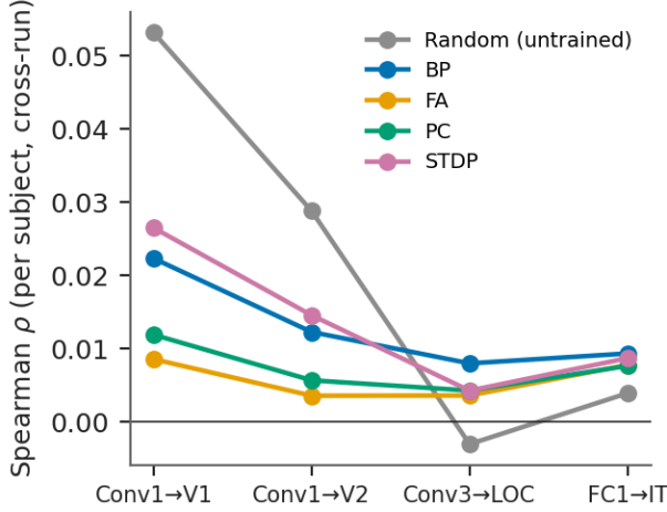
Figure 4: Brain alignment along the fixed layer-to-ROI mapping ( \rho_{\text{subj}} , cross-run). All conditions are lower at LOC than at V1. At IT the conditions lie between 0.004 and 0.009 and are not distinguishable. The untrained network is the highest at V1/V2 and the lowest at LOC and IT.
