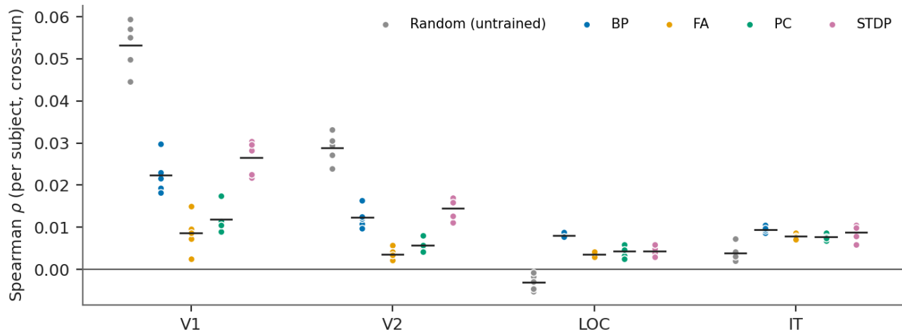
Figure 6: RSA scores of the 5 seeds per condition (dots) and their mean (line), \rho_{\text{subj}} , cross-run pairs. At V1/V2, between-rule differences are large relative to the seed spread. At IT, the seed spread is small, and the lack of significant differences reflects the stimulus-sampling uncertainty.
