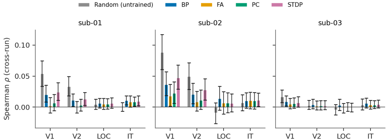
Figure 5: Single-subject RSA scores per learning rule and ROI (cross-run pairs, mean of 5 seeds), with stimulus-bootstrap 95% CIs. Sub-03 shows weaker alignment than sub-01 and sub-02 across conditions and ROIs. In sub-01 and sub-02 the V1 order of the point estimates is that of the group; at LOC, no difference between two trained rules is significant in any single subject.
