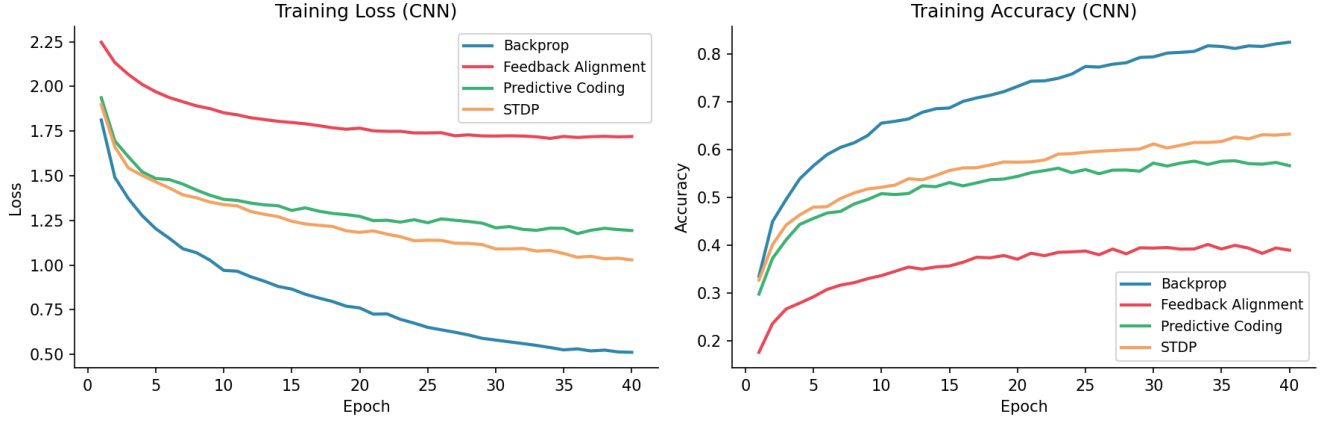
Figure 2: Training dynamics of the original runs: loss (left) and accuracy (right) on the training batches over 40 epochs (8,000 CIFAR-10 samples) for all four learning rules. All runs are stable without divergence. Test accuracies of the repaired models are in Table 1.
