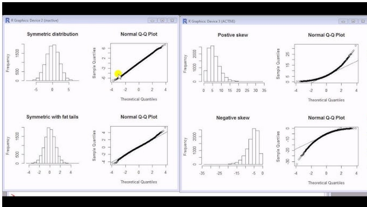
Figure 15: QQ-Plot Interpretation
