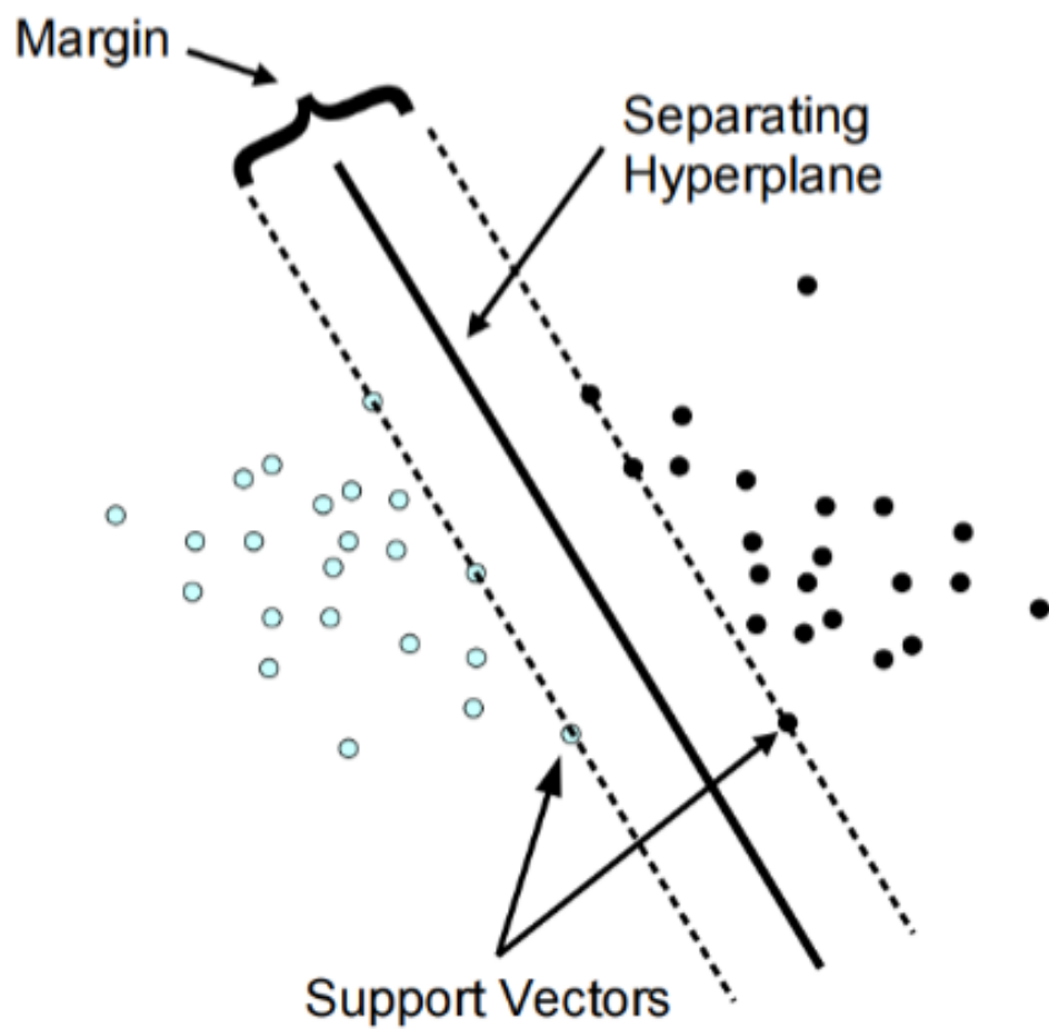
Figure 1: SVM
