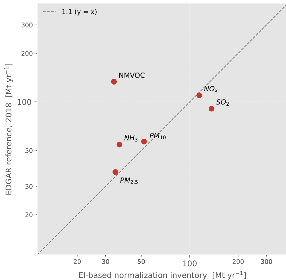
(b) Air pollutants
