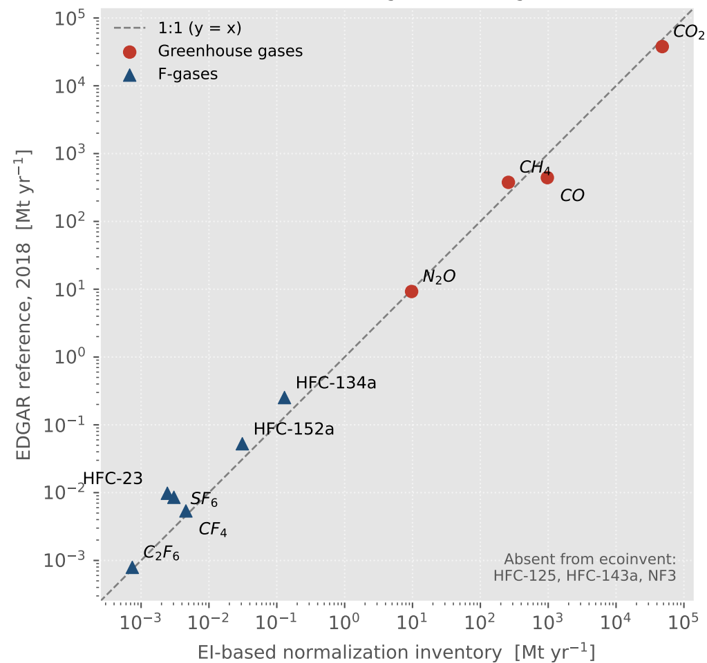
(a) Greenhouse gases and F-gases
