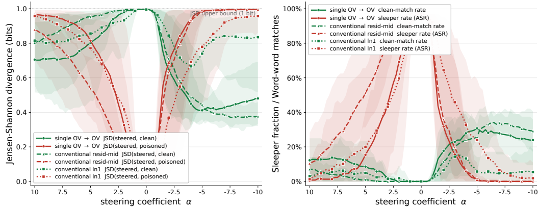
Figure 10: TinySleepers six-seed wide-coefficient screen. Solid circles: single OV→OV; dashed triangles: conventional resid-mid additive; dotted squares: conventional In1 additive. Left: JSD to the deployment-stripped clean baseline (green) and unsteered sleeper (red). Right: exact clean-rollout match rate (green) and sleeper-phrase ASR (red). Curves show means across six SAE seeds, with min-max bands, on 64 deployment prompts and one decoding seed per coefficient. Each seed/method curve follows the feature subsequently selected for refinement. Plotted \alpha = -\alpha_{\text{run}} ; the grid is [-10, 10] in steps of 0.25.
