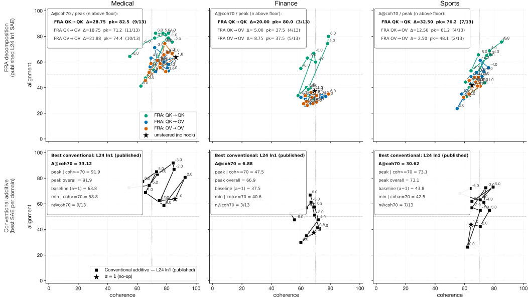
Figure 15: Alignment-coherence frontier per domain (columns: MEDICAL, FINANCE, SPORTS) at evaluation seed 42, over \alpha \in \{-6, \dots, 6\} . Top row : the three FRA recipes on the published L24 In1 SAE: QK→QK (green), QK→OV (blue), and OV→OV (orange). Bottom row : the best conventional additive recipe per domain (black), chosen by the largest \Delta alignment at coh \geq 70 among five SAEs (published L24 In1, L24 resid_pre/mid/post, L25 In1). Black stars mark the unsteered baseline; in the bottom row it sits at \alpha = 1 , where the additive update (\alpha-1) f W_{\text{dec}} vanishes. Each cell labels every \alpha point and reports peak, baseline, min|coh \geq 70 , and \Delta at coh \geq 70 . Negative \alpha pushes along the anti-feature direction and substantially extends the reachable alignment range, especially for the conventional recipe on MEDICAL.
