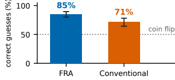
Figure 11: Autointerp of the steered TinyStories features. (a) Activation of each method's top-2 steering features on a triggered sentence; FRA's top feature fires only on the trigger. (b) Judge descriptions and accuracy for the top-5 features. (c) Mean accuracy over all 20 steered features per method (95% CI; dotted line is chance).
