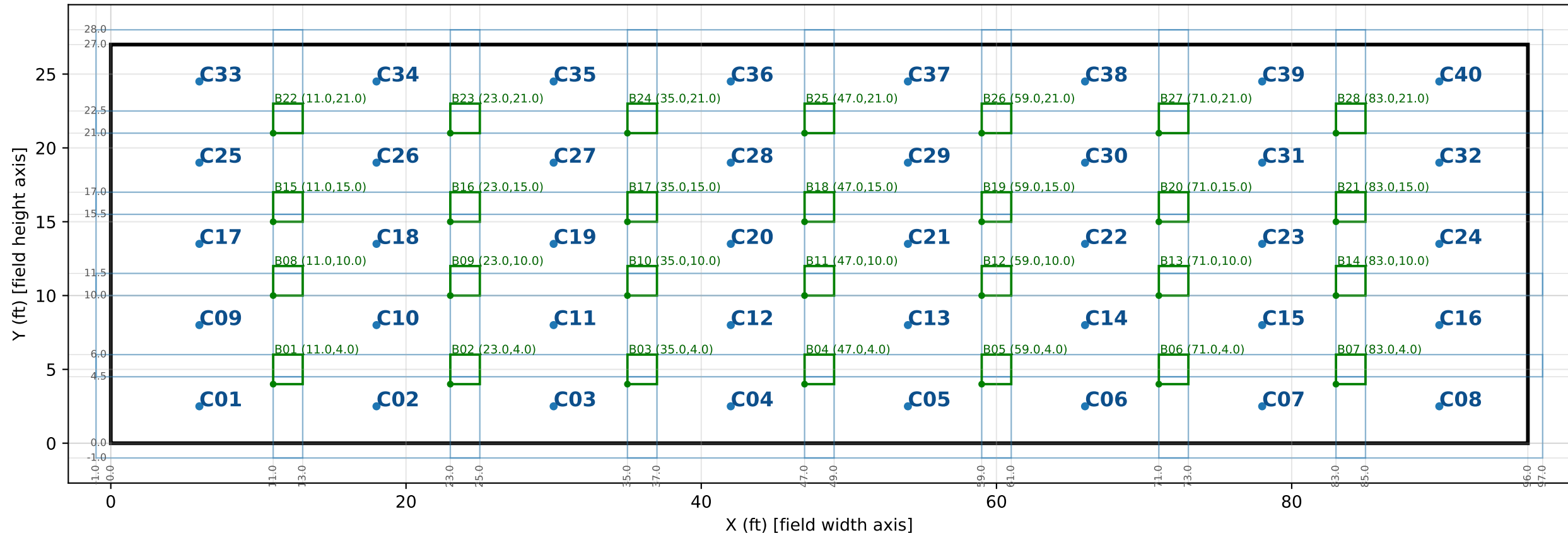
Camera Mesh and Board Placement Plan Origin: bottom-left, X rightward, Y upward
