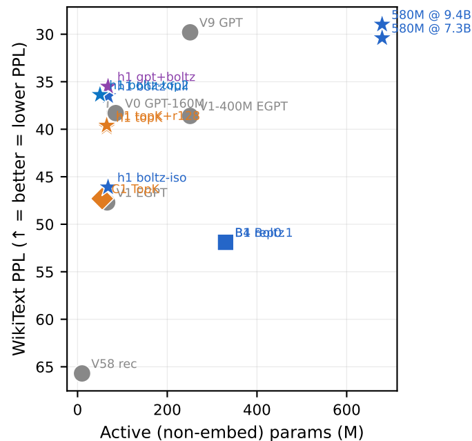
MoE variants vs baselines (7.86B tokens) x-axis: active (per-token) params — Boltzmann active=total; TopK active<total
