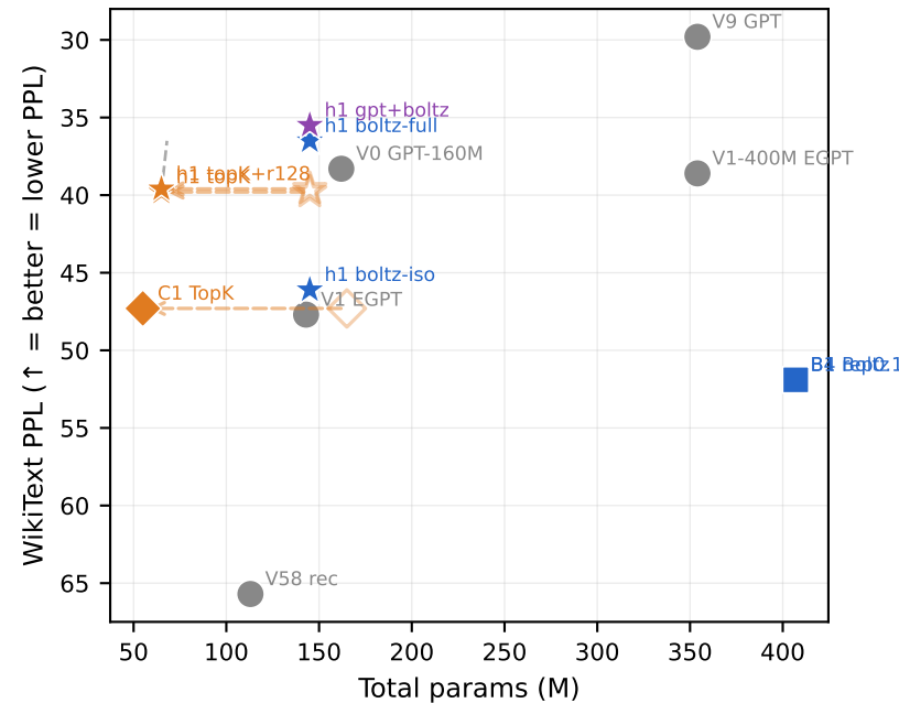
MoE variants vs baselines (7.86B tokens) x-axis: total params; dashed arrow shows sparsity discount for TopK models
