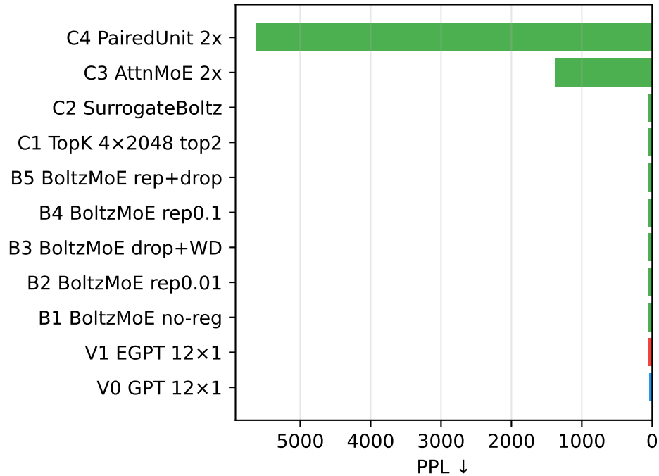
MoE series: PPL ↓
