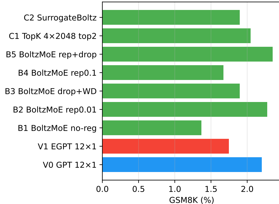
MoE series: GSM8K (%)
