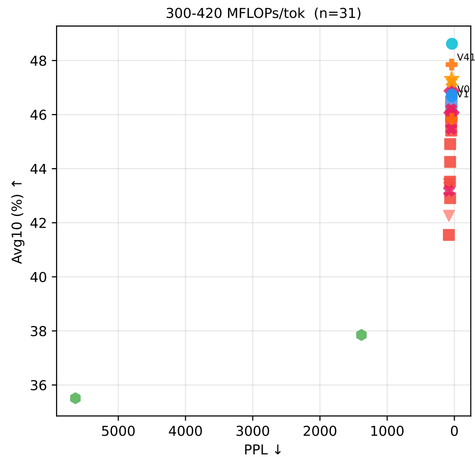
PPL vs Accuracy at matched FLOPs/token
