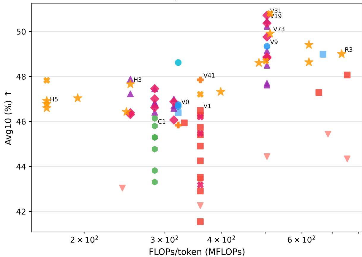
Accuracy vs. FLOPs/token
