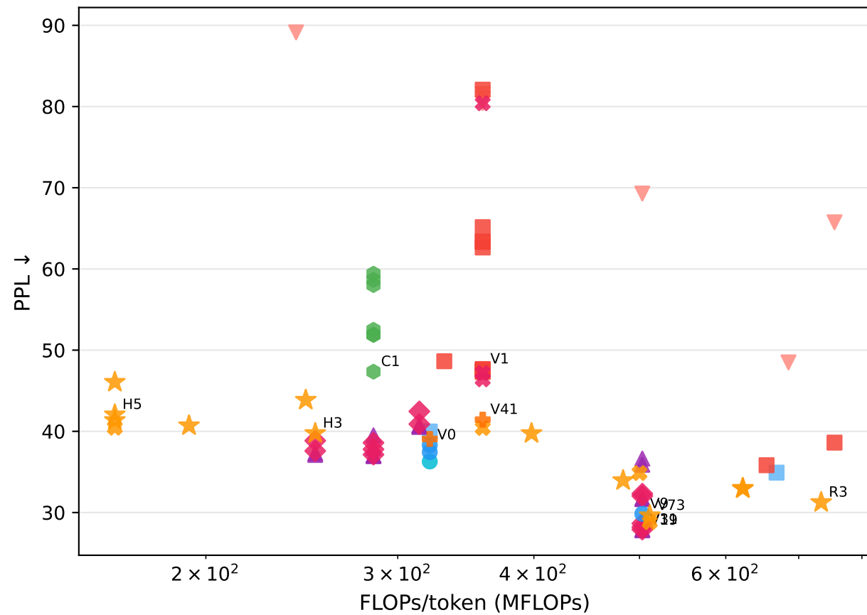
PPL vs. FLOPs/token
