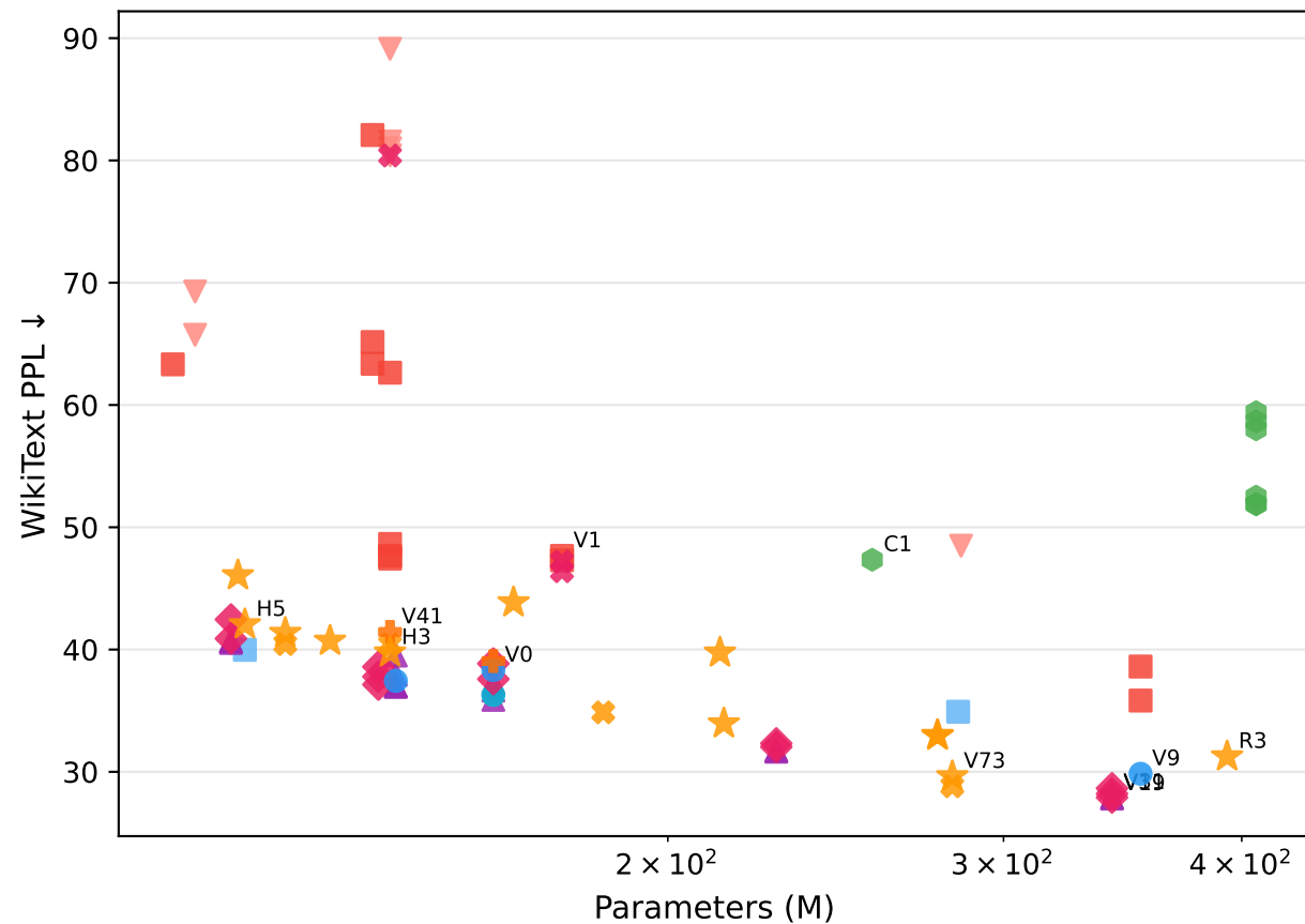
PPL vs. Parameters (MoE outliers PPL>100 omitted)
