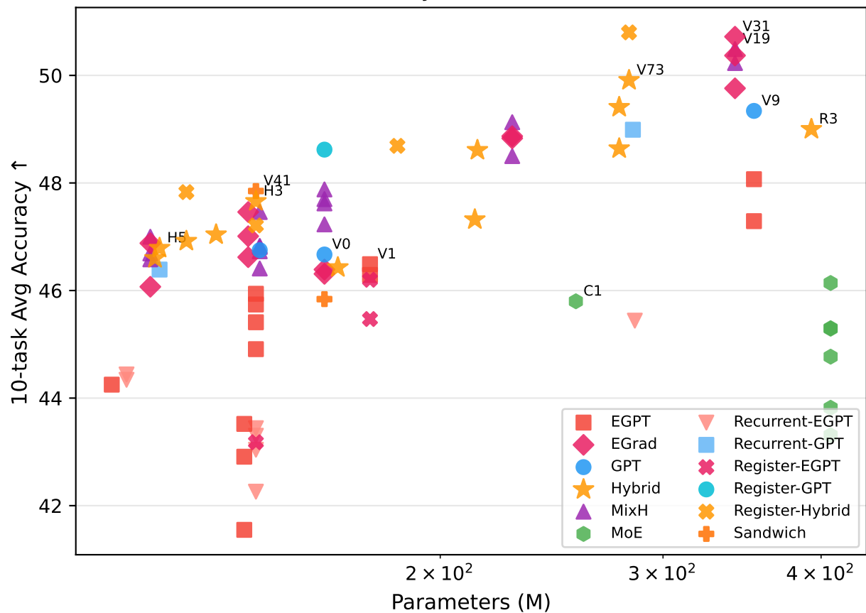
Accuracy vs. Parameters
