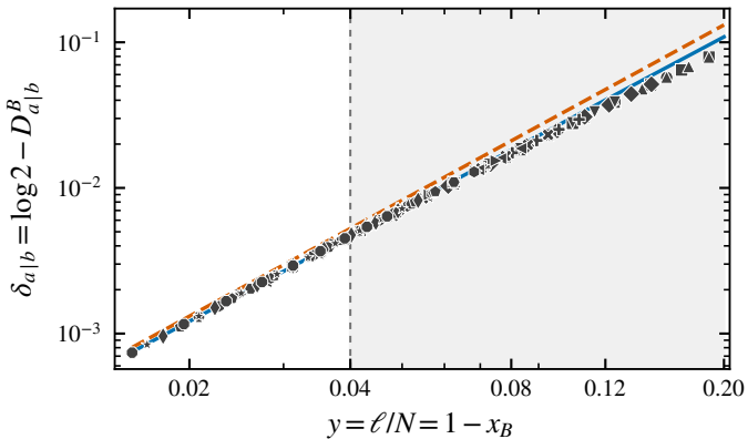
(e) ss|3s,s
