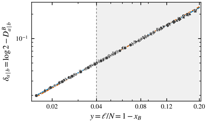
(c) 00|3s,s
