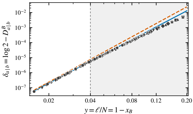
(e) ss|3s,s
