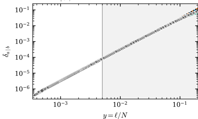
(e) \delta_{ss|3s,s}
