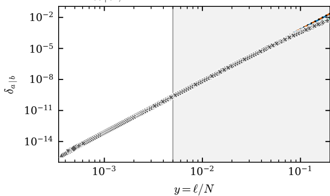
(e) \delta_{ss|3s,s}
