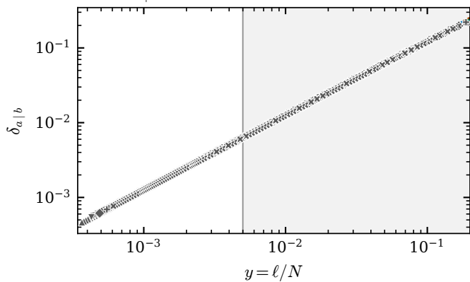
(c) \delta_{00|3s,s}
