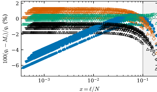
(e) D_{ss|3s,s}^A
