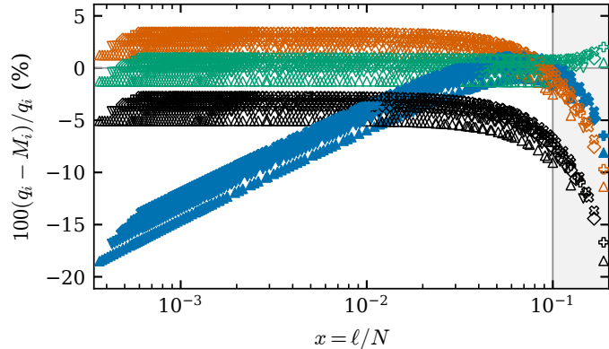
(f) D_{3s,s|ss}^A
