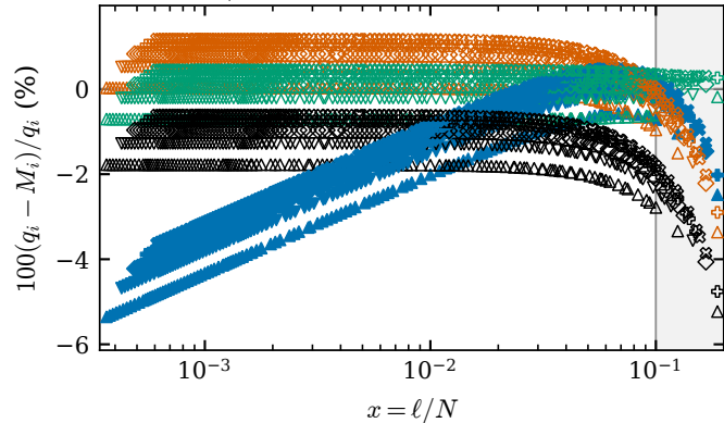
(f) D_{3s,s|ss}^A
