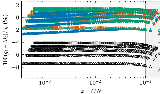
(c) D_{00|3s,s}^A
