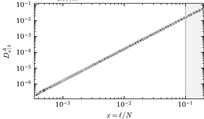
(f) D_{3s,s|ss}^A
