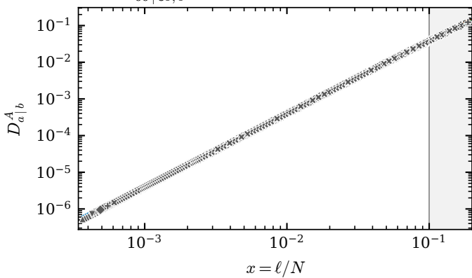
(e) D_{ss|3s,s}^A
