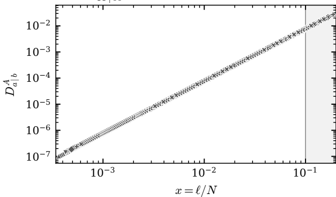
(c) D_{00|3s,s}^A
