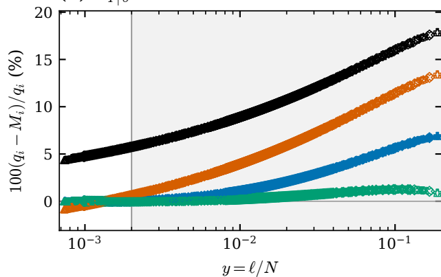
(c) \delta_{I|\varepsilon}
