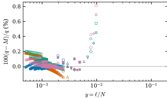
(e) \sigma | \varepsilon
