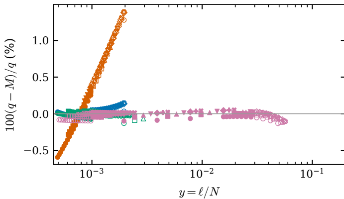
(c) I | \varepsilon
