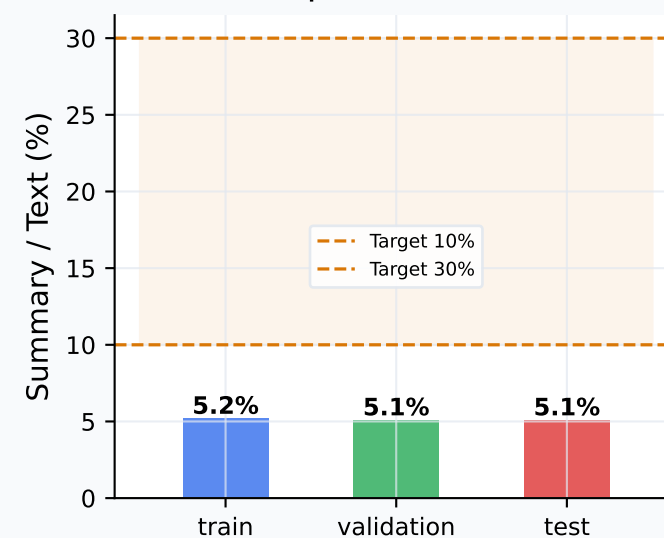
Compression Ratio
