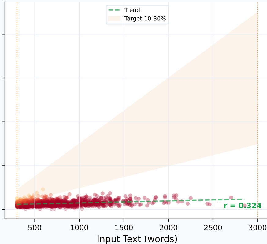
Validation (n=2,000)
