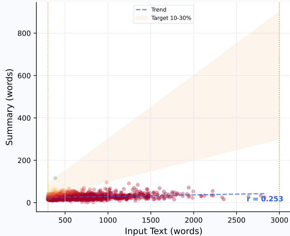
Train (n=2,000)
