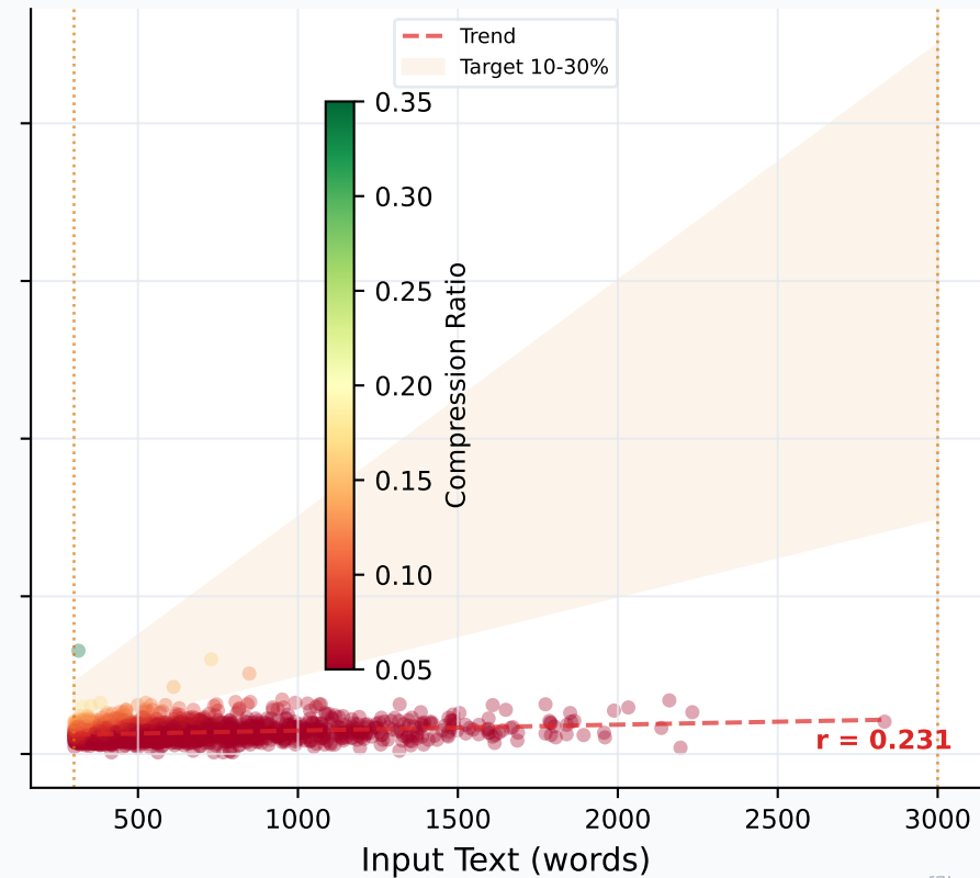
Test (n=2,000)
