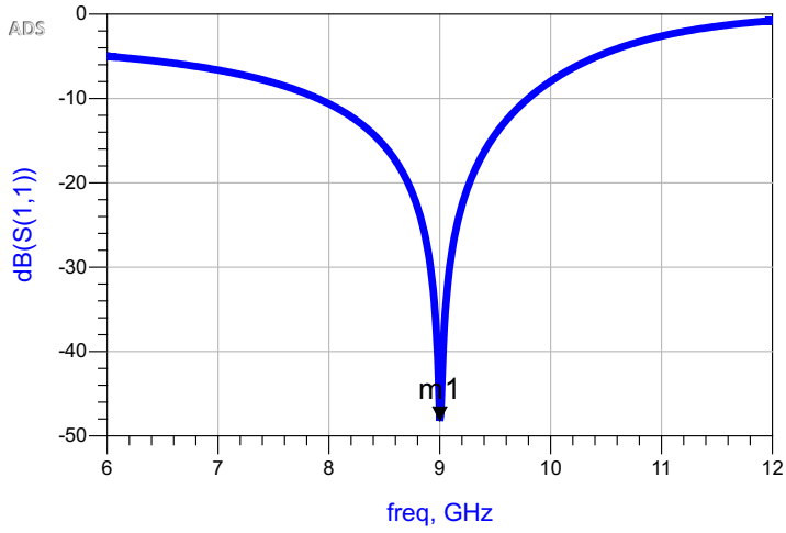
Impedance Validation of the 50-Ohm Transmission Line
