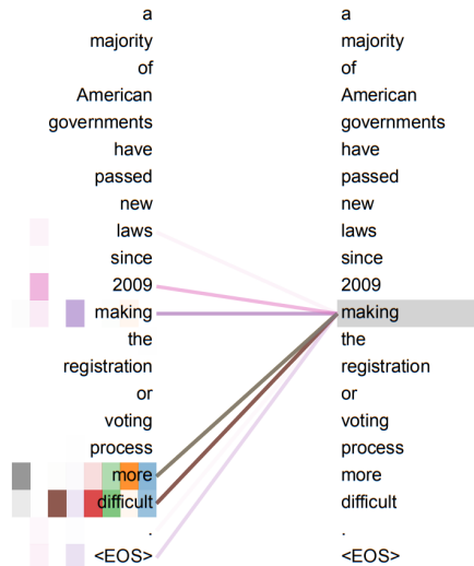
Figure adapted from Ashish Vaswani et al. Attention is All You Need paper
