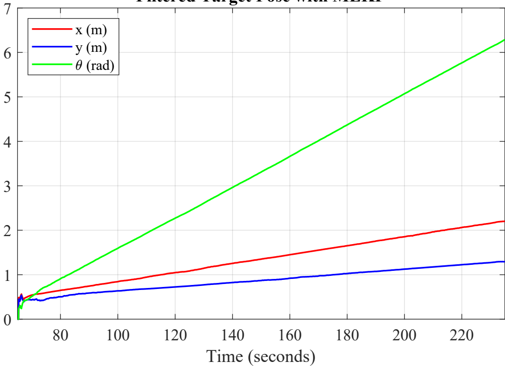
Filtered Target Pose with MEKF
