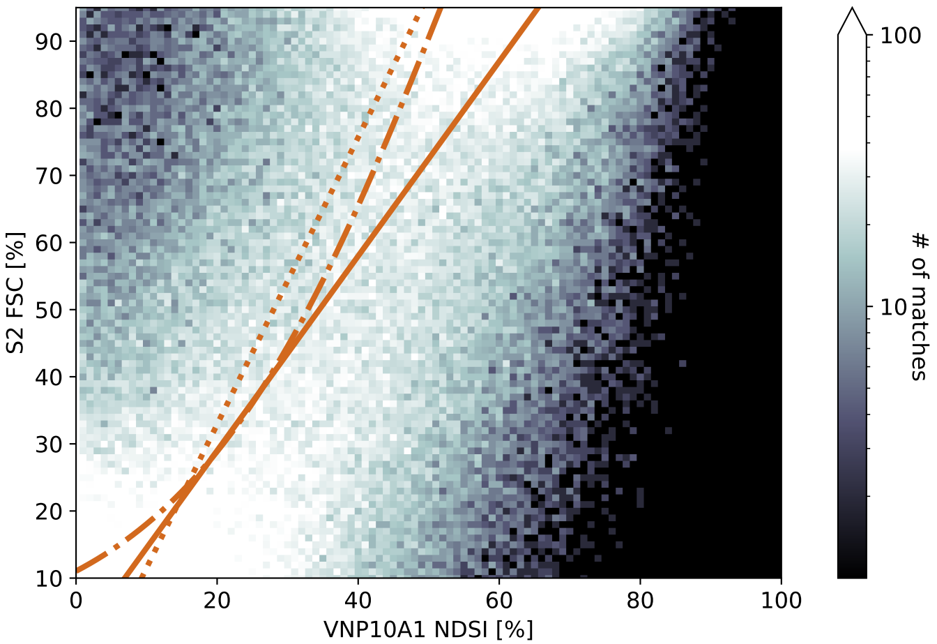
Forest r=0.56
