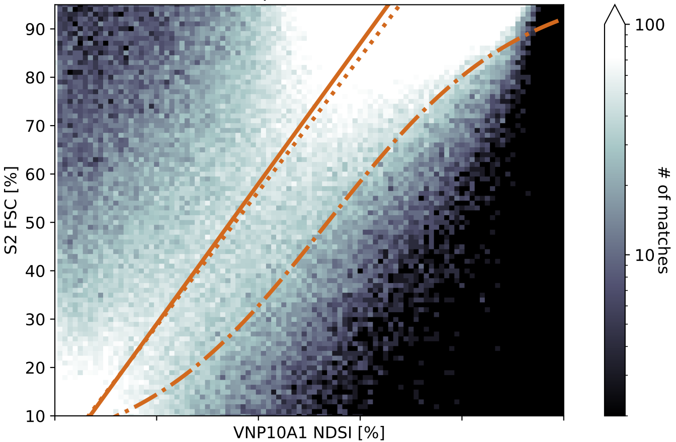
Open r=0.75
