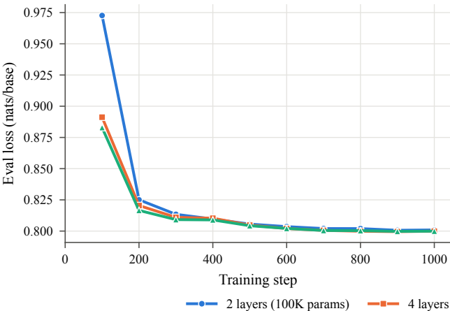
(a) Eval loss
